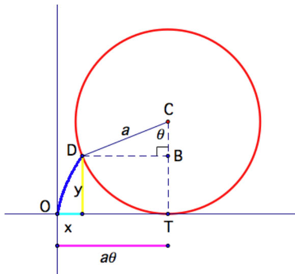
Figure 4: Finding the Coordinates of the Point D on a Cycloid
