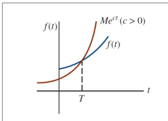
Figure 3: f is of exponential order with constants c, M and T
