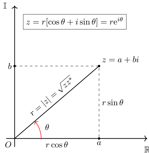
Figure 1: The Complex Plane
