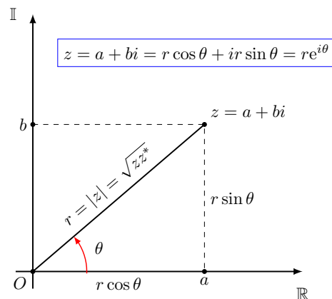
Figure 1: The Complex Plane
